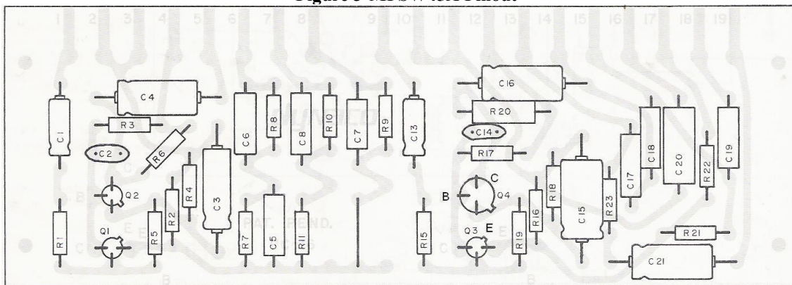
Figure 4-circuit board as seen from solder side. The modification replaces Q4
