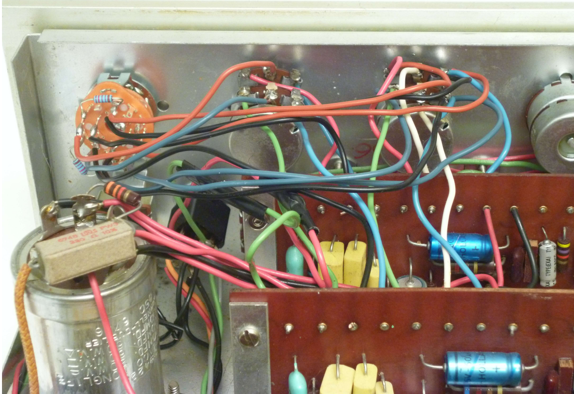
Figure 7-Tone control switch installed and wired to bass control, treble control and PCB's (green wires called out in the assembly directions are blue in the pictures above).
